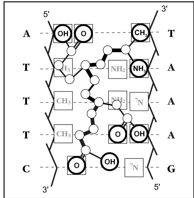
Figure 4. Model of complementary interaction of the peptide Ala-Glu-Asp-Gly with DNA double-helix (DNA-peptide complex on the promoter region of telomerase gene).
