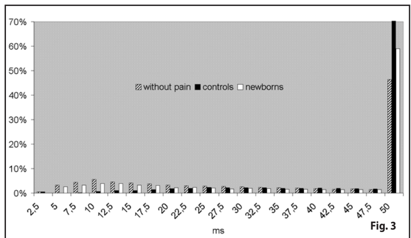
Figure 3: Histogram of interspike intervals in two experimental groups (newborn: deafferentation performed in infant rats; without pain: non-mutilating deafferentated rats from the adult group) and in control animals. Distributions of ISIs is almost the same in two experimental groups suggesting functionally similar neural network in both groups.
